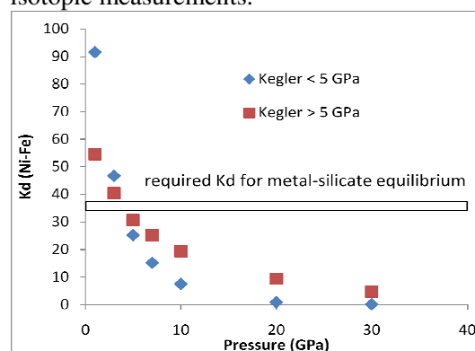
Figure 1: K_d(\text{Ni-Fe}) met/sil vs. pressure calculated for high pressure >5 GPa and low pressure ( < 5 GPa) data of [5]. K_d(\text{Ni-Fe}) of 33 is required for equilibrium in the Mars mantle, which is best matched near 4 GPa and 2373 K.
